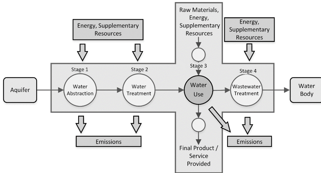
Figure 1. Generic meso-level water system
